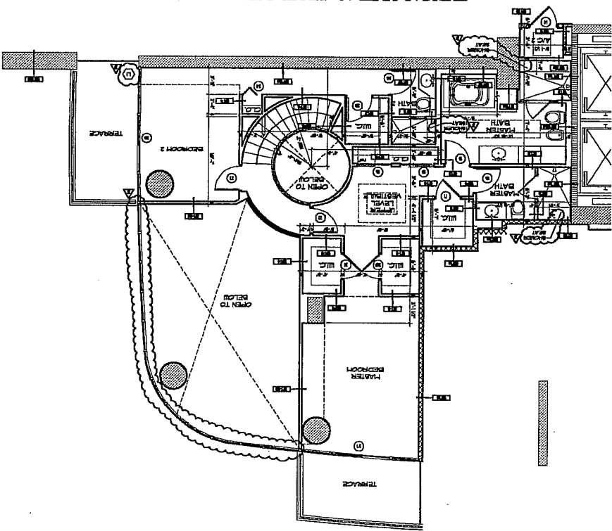
TYPICAL UNIT-19 UPPER LEVEL FLOOR PLAN (7TH AND 9TH FLOORS - SOUTH TOWER) SCALE: 1/8" = 1'-0"
