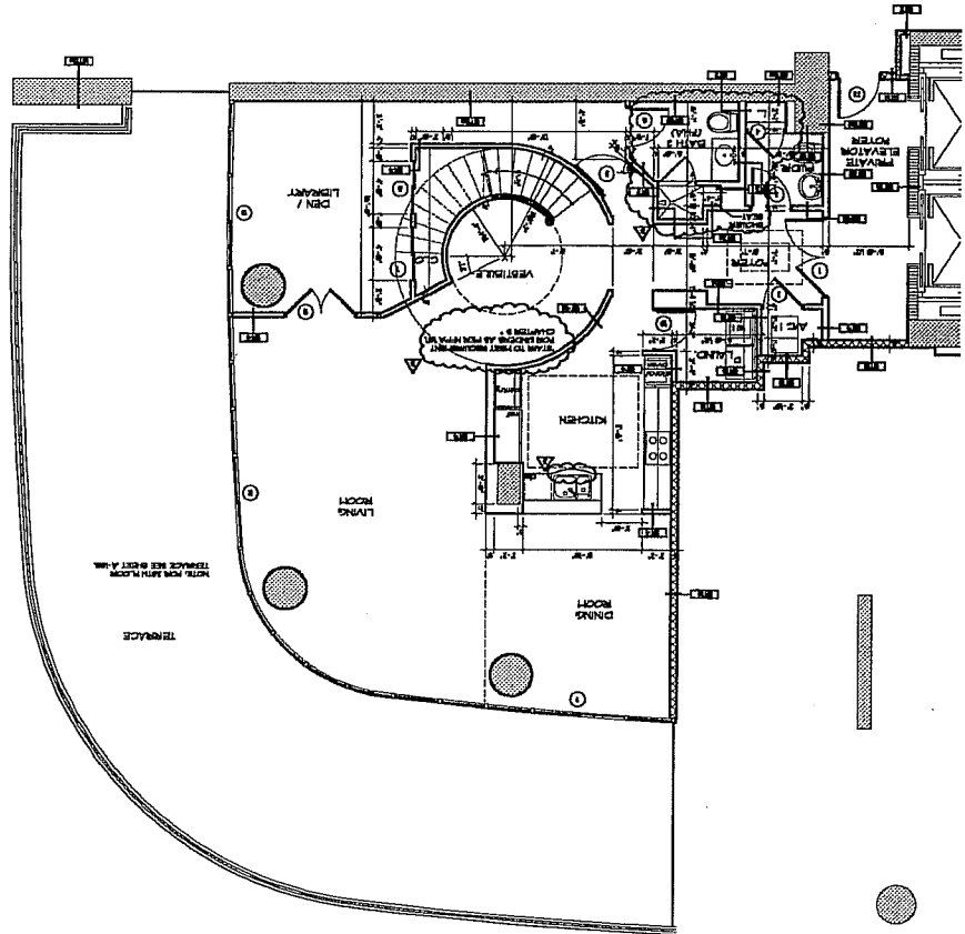
TYPICAL UNIT-19 LOWER LEVEL FLOOR PLAN (6TH FLOOR - SOUTH TOWER) (8TH FLOOR SIMILAR) SCALE: 1/8" = 1'-0"
